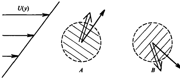
FIGURE 3. Propagation of two wave packets A and B in shear flow. Lines show wavecrests, single arrows wavevectors, and double arrows the group-velocity vectors.
