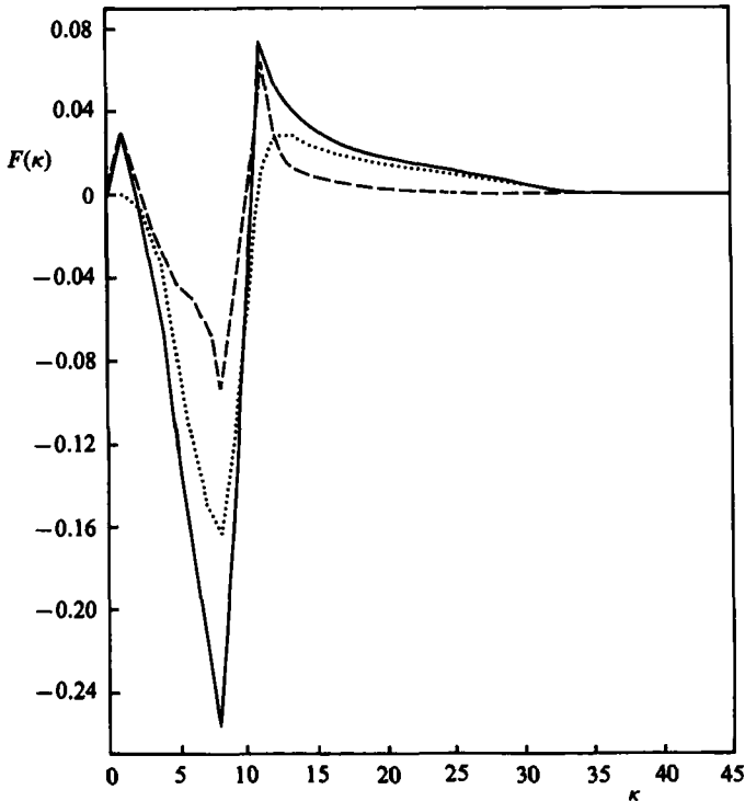
FIGURE 19. Time-averaged spectral fluxes of energy, run D: F_{ST}(\kappa) (---), F_T(\kappa) (.....), and F(\kappa) (—).
