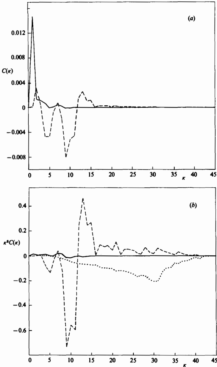
FIGURE 13. (a) Energy conversion terms C_S(\kappa) (—) and C_T(\kappa) (---), and (b) entrophy conversion terms \kappa^2 C_S(\kappa) (—) and \kappa^2 C_T(\kappa) (---), for run C, averaged over t = 0-15 . In (b) the dotted line shows the time-averaged dissipation of entrophy, which outside of the initial scales 9 \leq \kappa < 12 must be balanced by nonlinear transfer less net accumulation.
