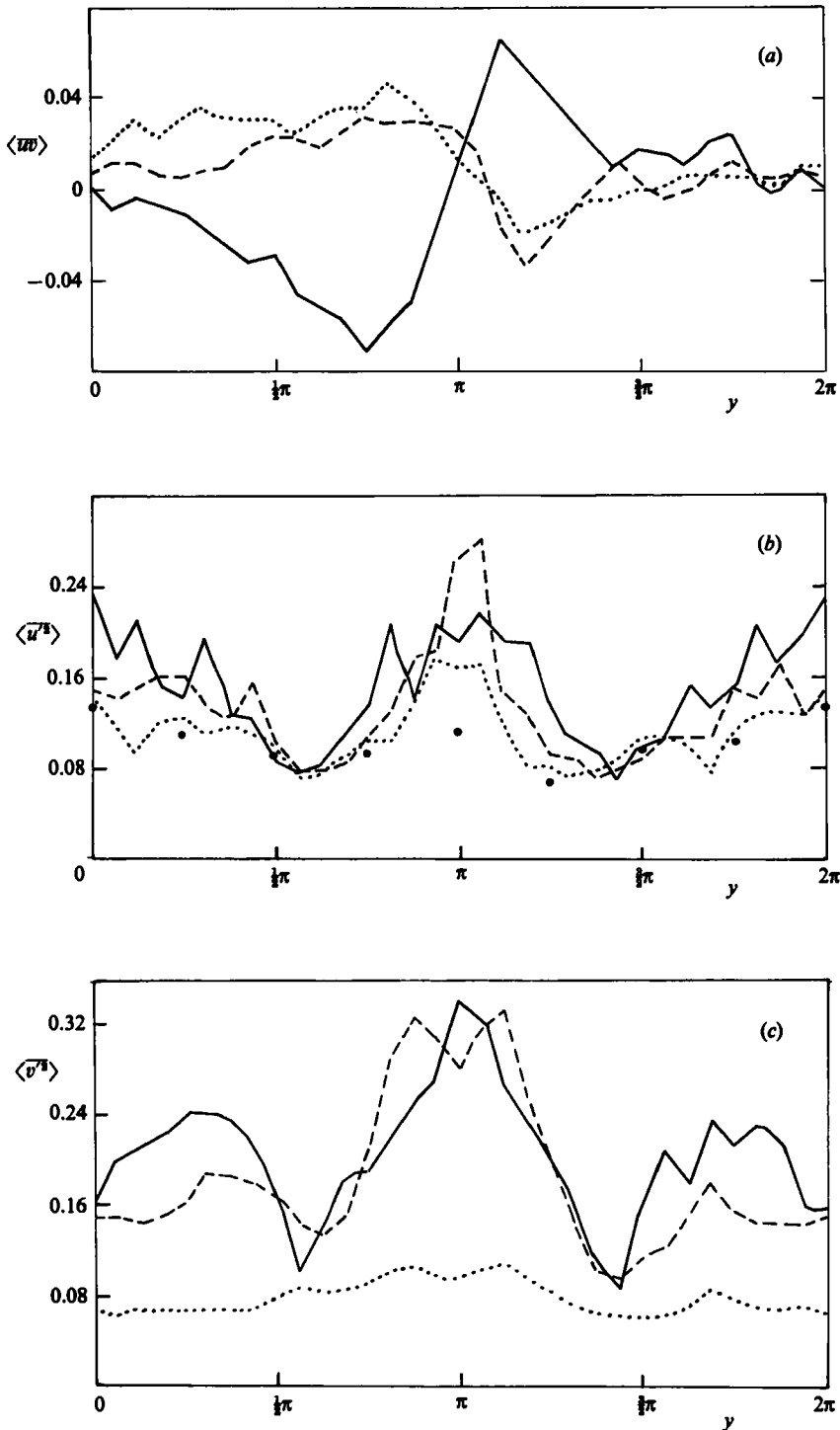
FIGURE 15. Ensemble average of x -averaged spatial diagnostics from run C and two similar runs, time-averaged over t = 0-1 (—), t = 1-2 (---), and t = 0-15 (····). (a) \langle \overline{w\overline{w}} \rangle(y) (here the t = 0-15 values have been multiplied by 5 to be visible); (b) \langle \overline{u^2} \rangle(y) ; (c) \langle \overline{v^2} \rangle(y) . The large dots in (b) show, for selected y , the contribution from zonal-wave ( k \neq 0 ) modes for t = 0-15 .
